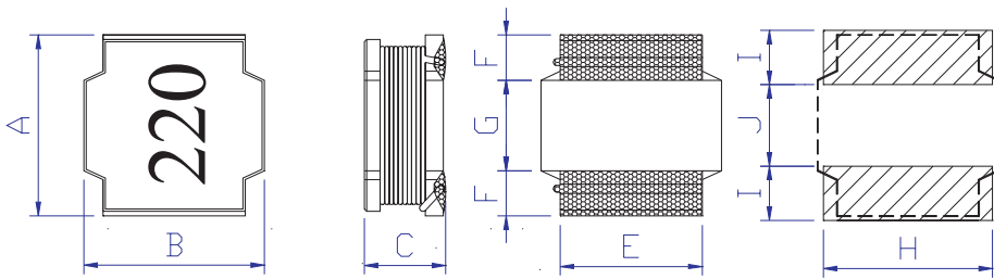
Land Pattern
